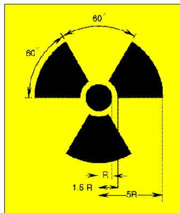
RADIATION SYMBOL
