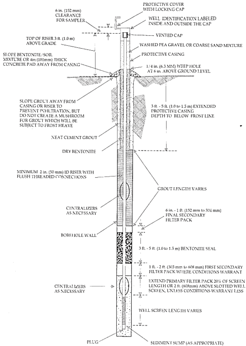
Figure 2. Monitoring Well Design - Single Cased Well
