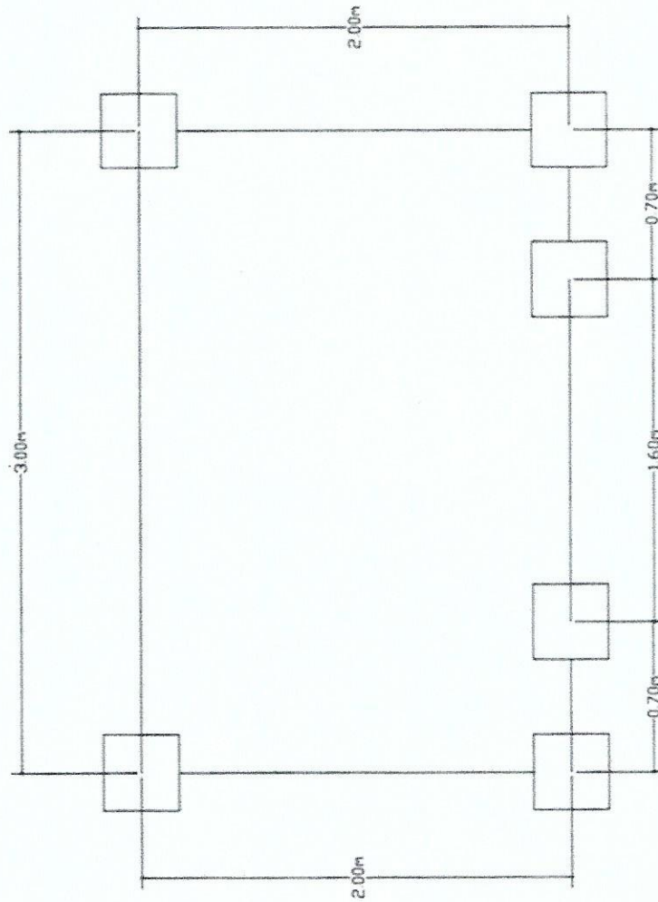
FOUNDATION PLAN
