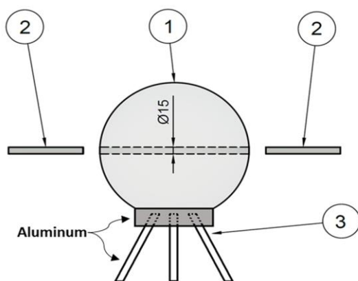
Figure 2. Illustration of the (1) sphere with (2) plugs and (3) aluminum base support. The aluminum support is composed of 4 aluminum rods threaded into an aluminum base.
