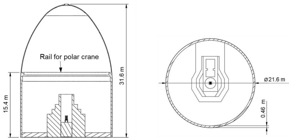
Figure 1 Reactor dome (dimensions in m)
