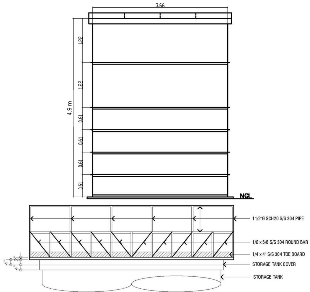
Figure 3 Fuel storage tank (dimensions in m) with bridge (English units)
