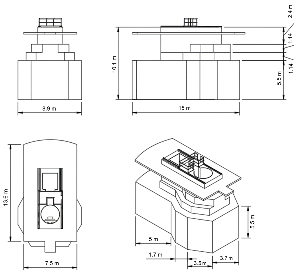
Figure 2 Reactor pool (dimensions in m)
