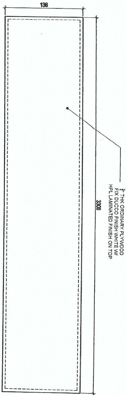
1 TOP VIEW SCALE 1:20 MTS
