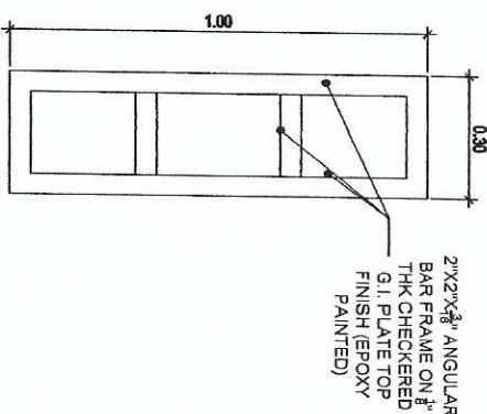
3 DETAILS OF STEP FRAME SCALE NTS
