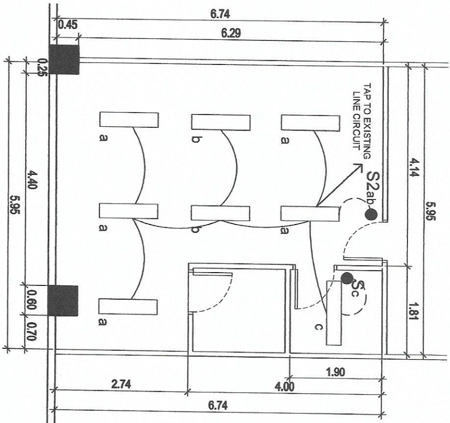
NSD CHIEF OFFICE
