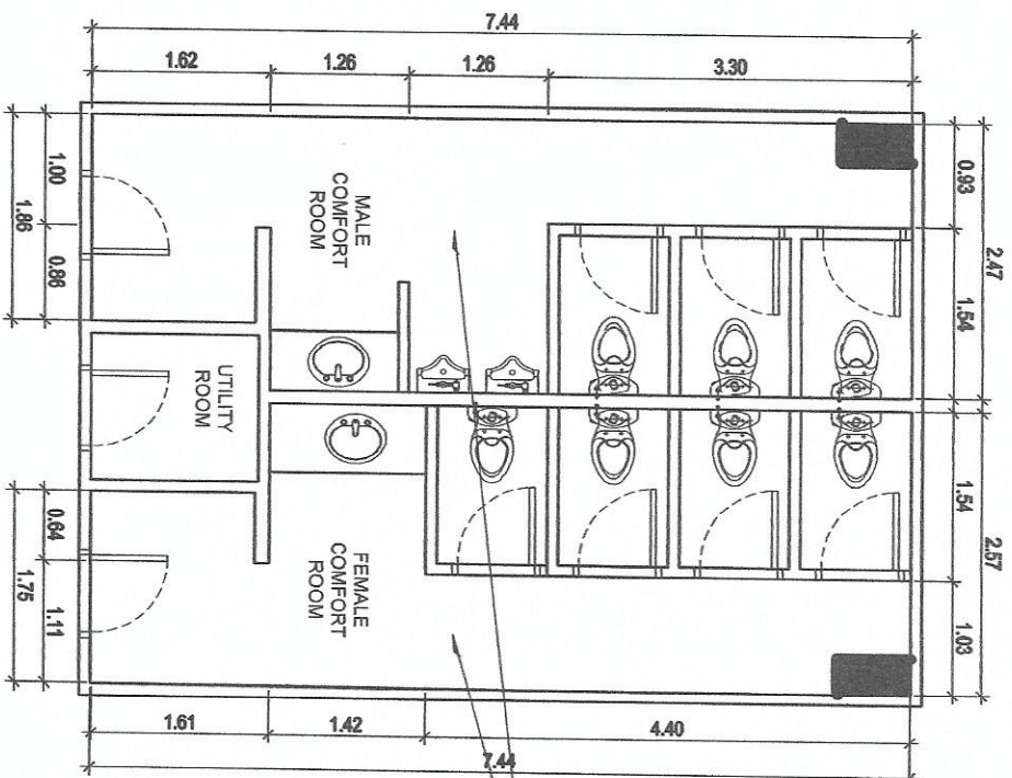
SECOND FLOOR RIGHT WING PUBLIC COMFORT ROOM
