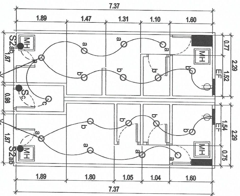
GROUND FLOOR LEFT WING PUBLIC COMFORT ROOM
