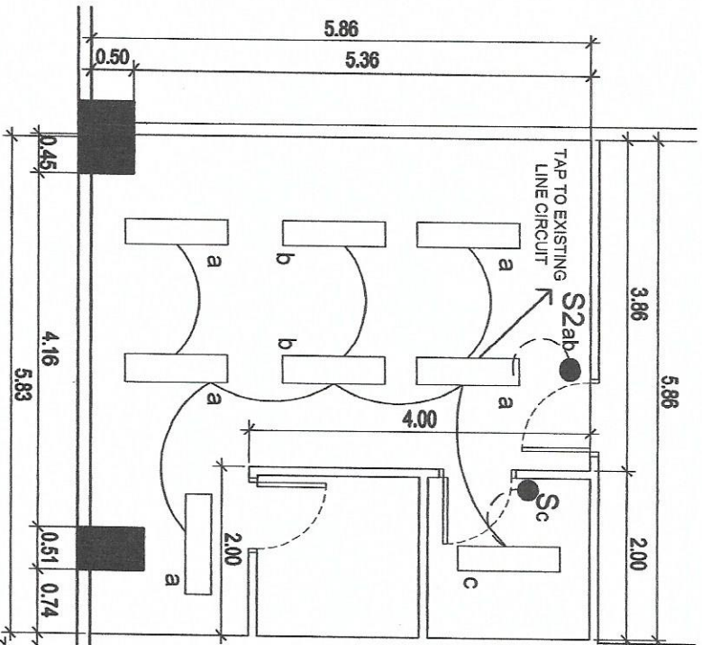
NRD CHIEF OFFICE
