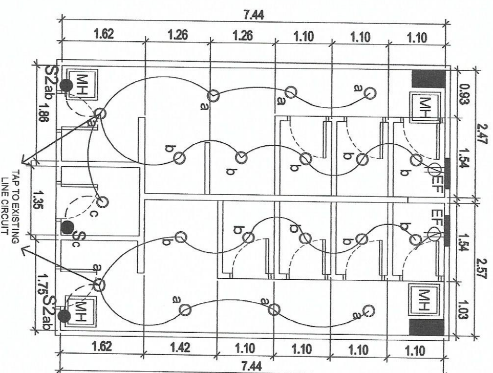
SECOND FLOOR RIGHT WING PUBLIC COMFORT ROOM
