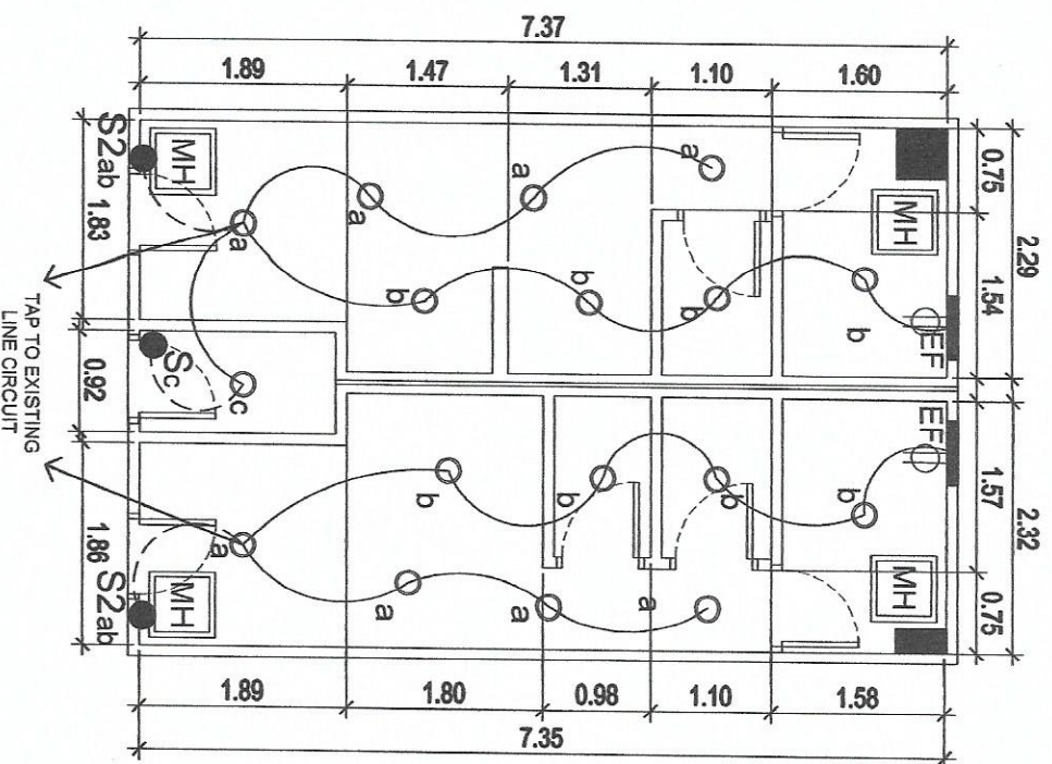
SECOND FLOOR LEFT WING PUBLIC COMFORT ROOM
