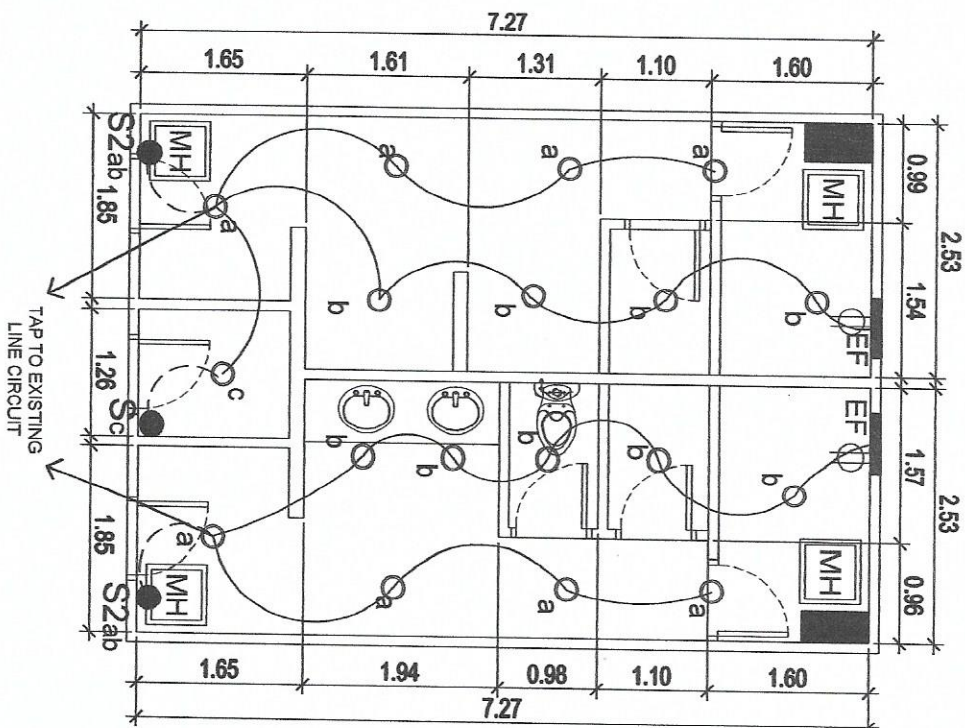
THIRD FLOOR RIGHT WING PUBLIC COMFORT ROOM
