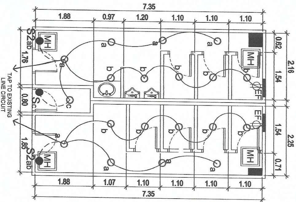
THIRD FLOOR LEFT WING PUBLIC COMFORT ROOM
