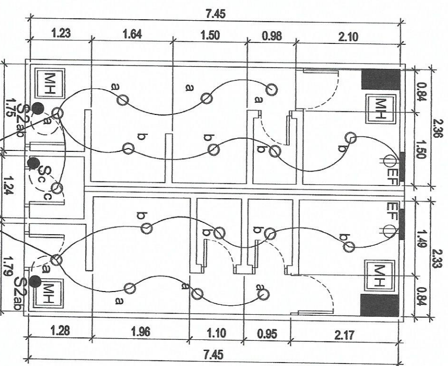
GROUND FLOOR RIGHT WING PUBLIC COMFORT ROOM
