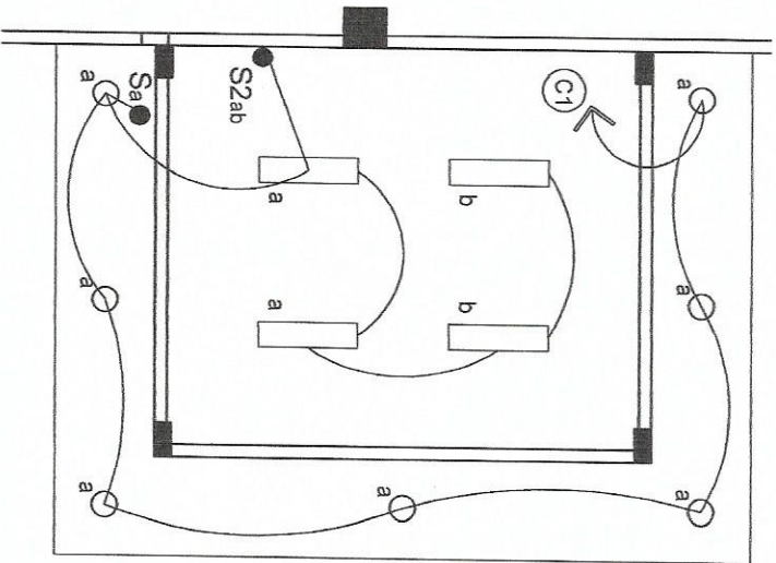
LIGHTING LAYOUT PLAN
