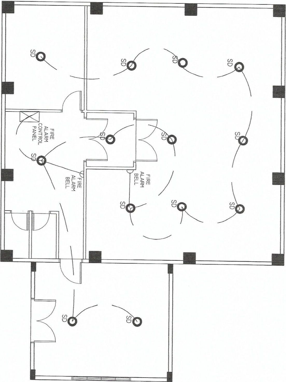
SMOKE DETECTOR LAYOUT
