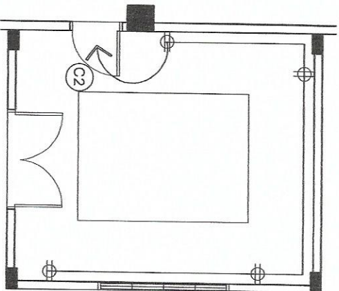
POWER LAYOUT PLAN
