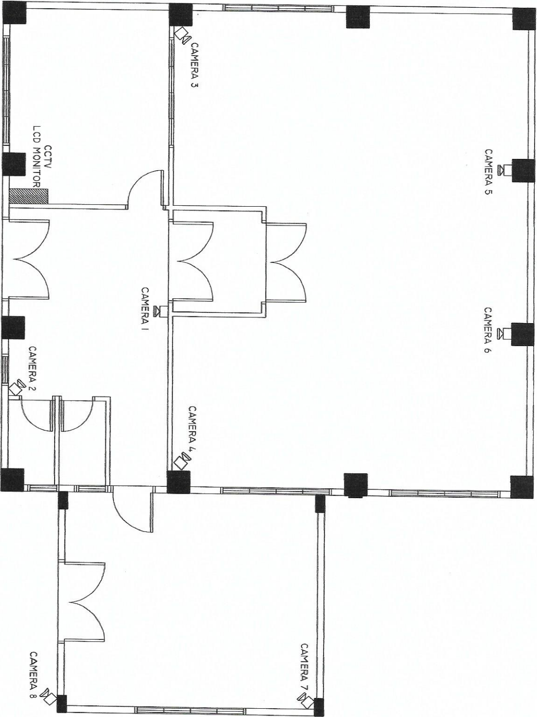
CCTV CAMERA LAYOUT
