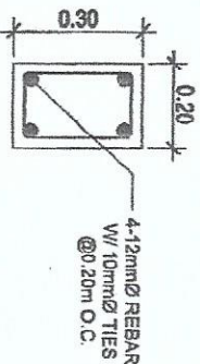
2 TIE BEAM DETAIL (TB) SCALE 1:16 MTS
