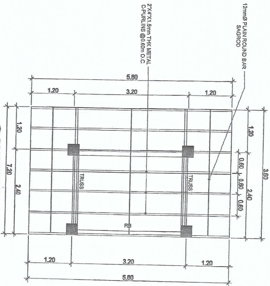
2 ROOF FRAMING PLAN SCALE 1:80 MTS
