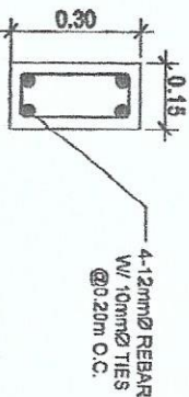
3 ROOF BEAM DETAIL (RB) SCALE 1:16 MTS
