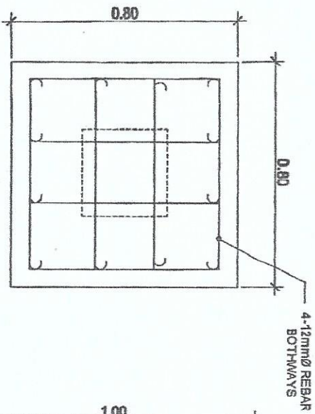
1 COLUMN DETAIL (C-1) SCALE 1:16 MTS
