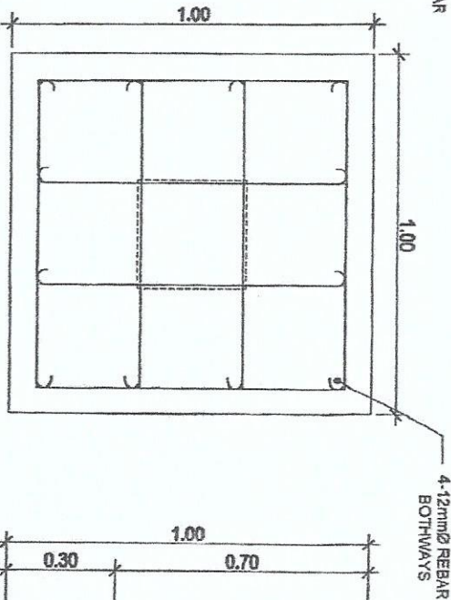
5 FOOTING DETAIL (F-2) SCALE 1:16 MTS
