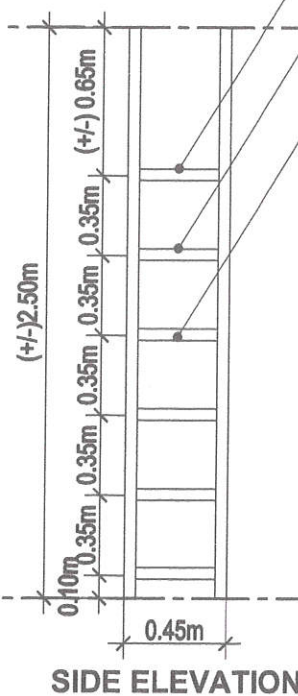
1 TYPICAL DETAIL OF BUILT-IN OPEN STEEL SHELVES SCALE NTS
