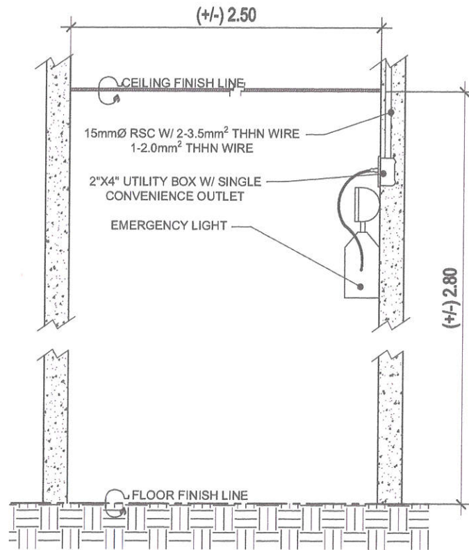
1 SCALE TYPICAL INSTALLATION OF EMERGENCY LIGHT NTS
