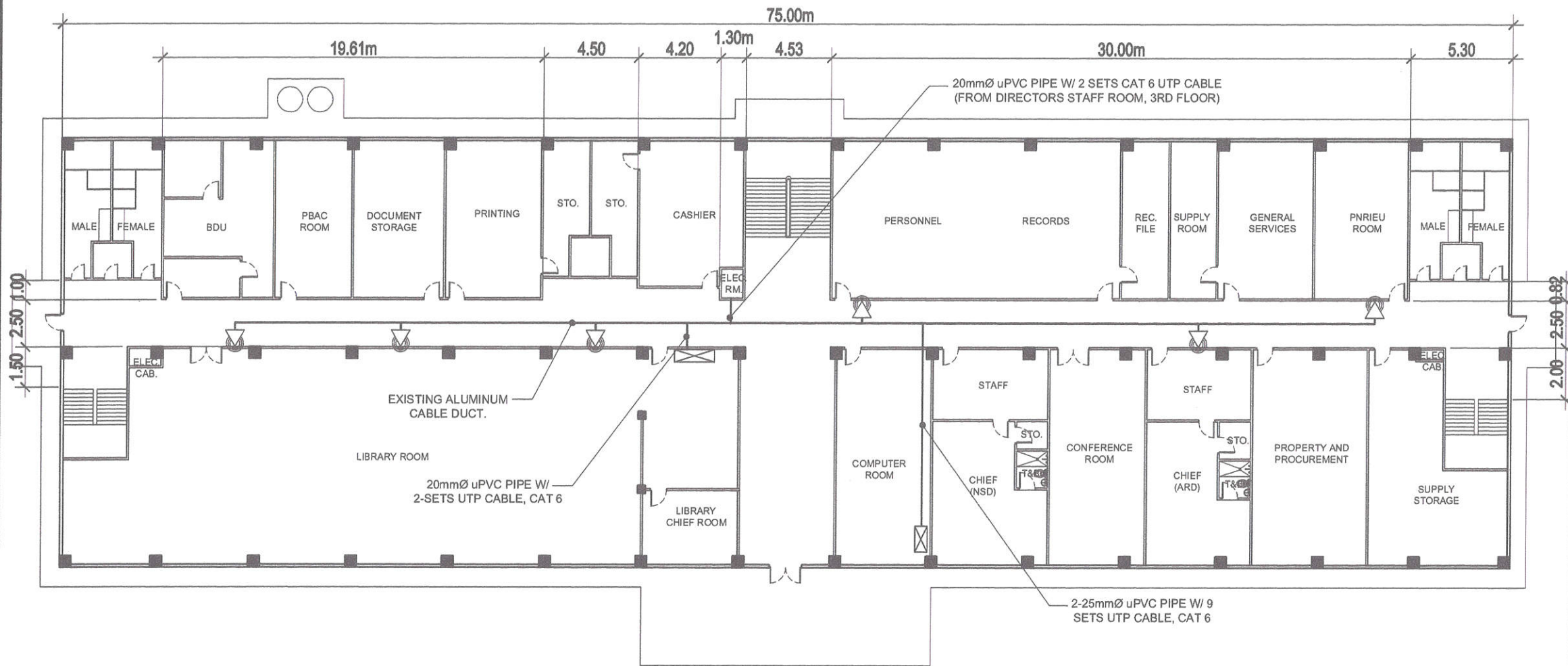
1 SECOND FLOOR PLAN (DATA LAN LAYOUT) SCALE NTS
