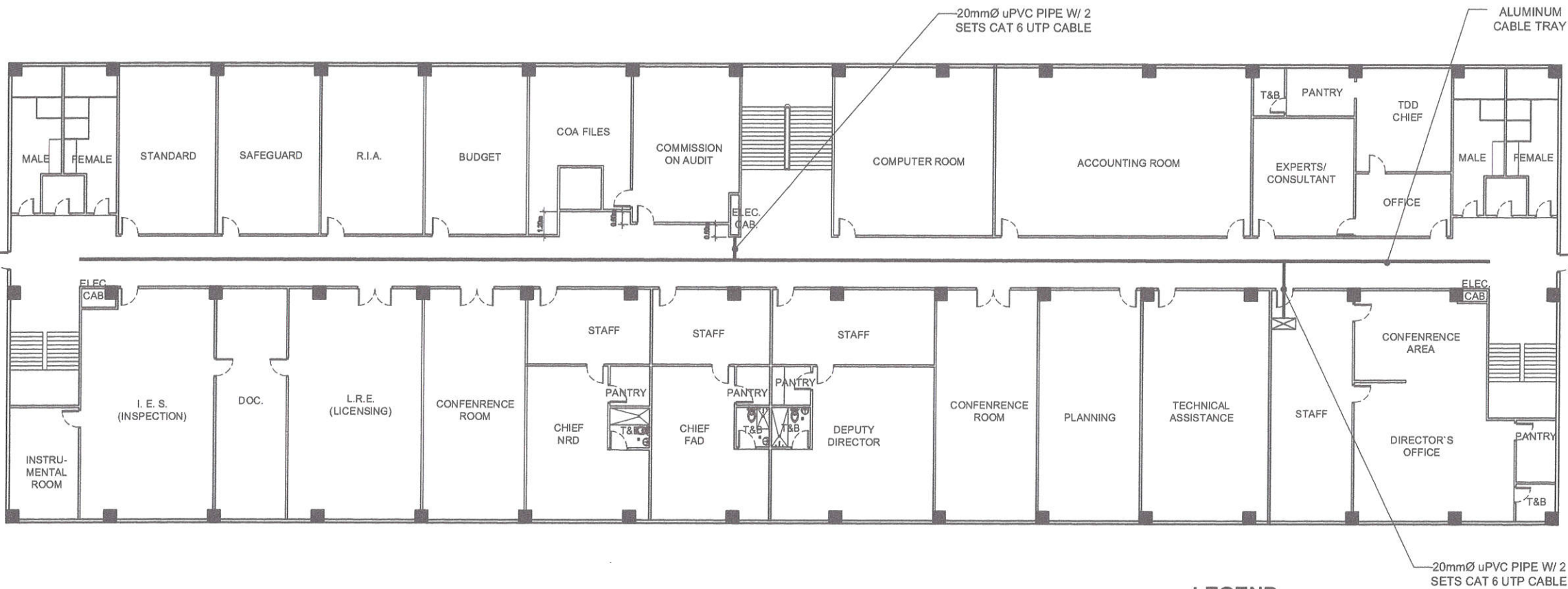
1 THIRD FLOOR PLAN (DATA LAN LAYOUT) SCALE _____ NTS
