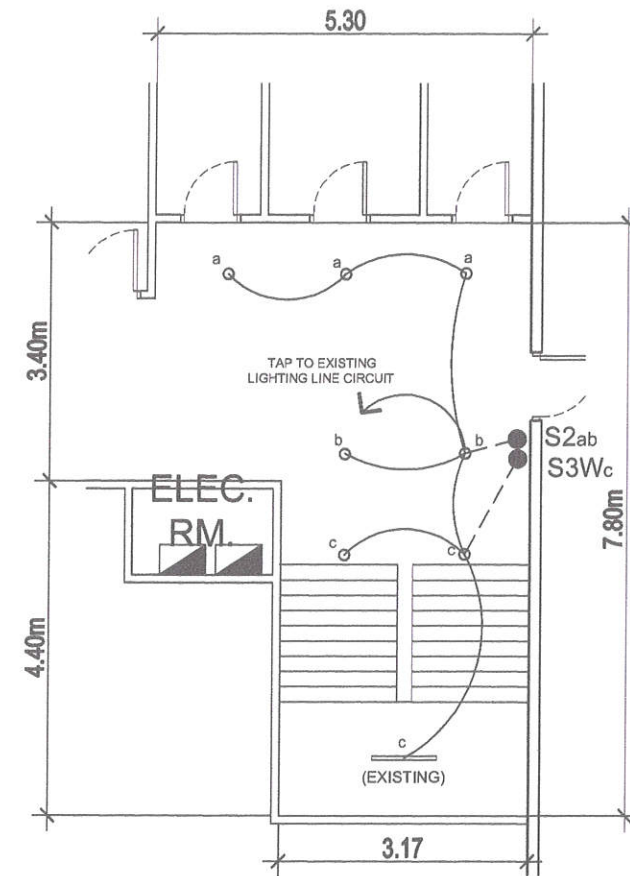
3 RIGHT WING SECOND FLOOR PLAN SCALE NTS
