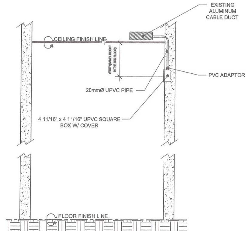
1 SCALE TYPICAL INSTALLATION FOR LAN ACCESS POINT NTS
