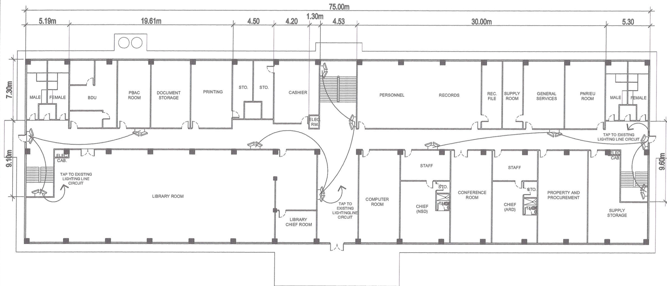
1 SECOND FLOOR PLAN - EMERGENCY LIGHT LAYOUT SCALE NTS
