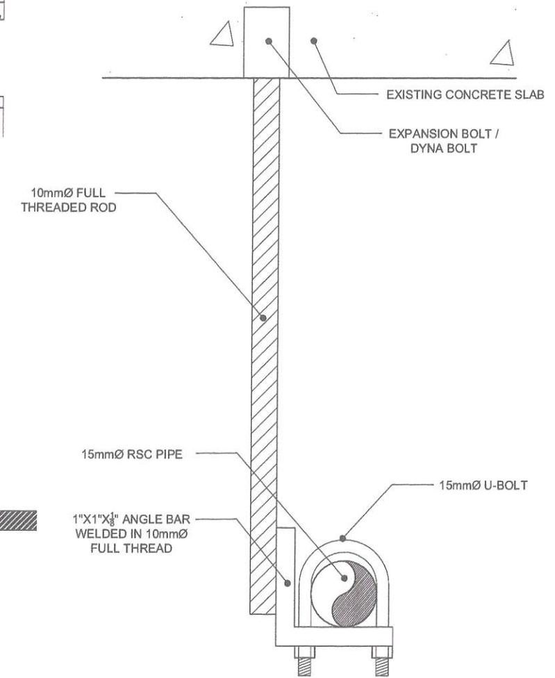
2 TYPICAL RSC HANGER/SUPPORT
