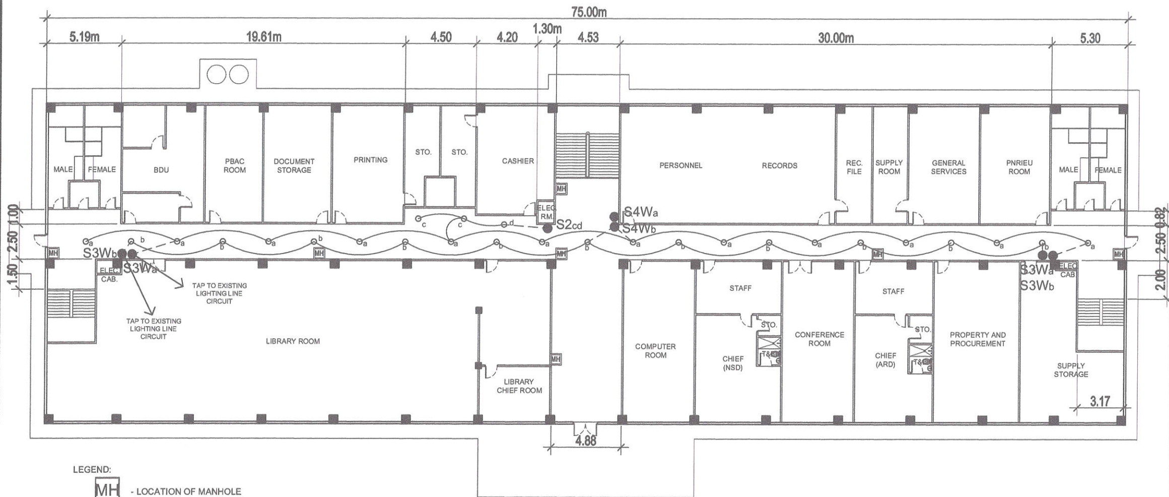
1 SECOND FLOOR HALLWAY LIGHTING LAYOUT SCALE NTS
