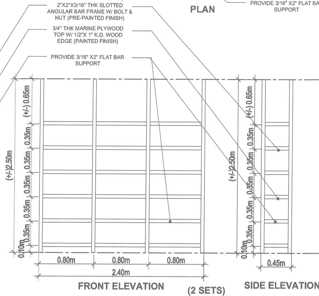
1 TYPICAL DETAIL OF BUILT-IN OPEN STEEL SHELVES SCALE NTS
