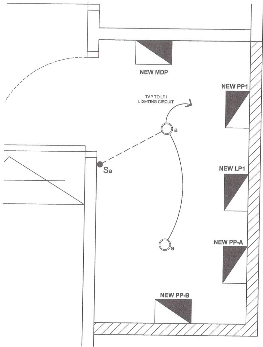
1 EXTENSION OF ELECTRICAL ROOM (LIGHTING LAYOUT) SCALE NTS
