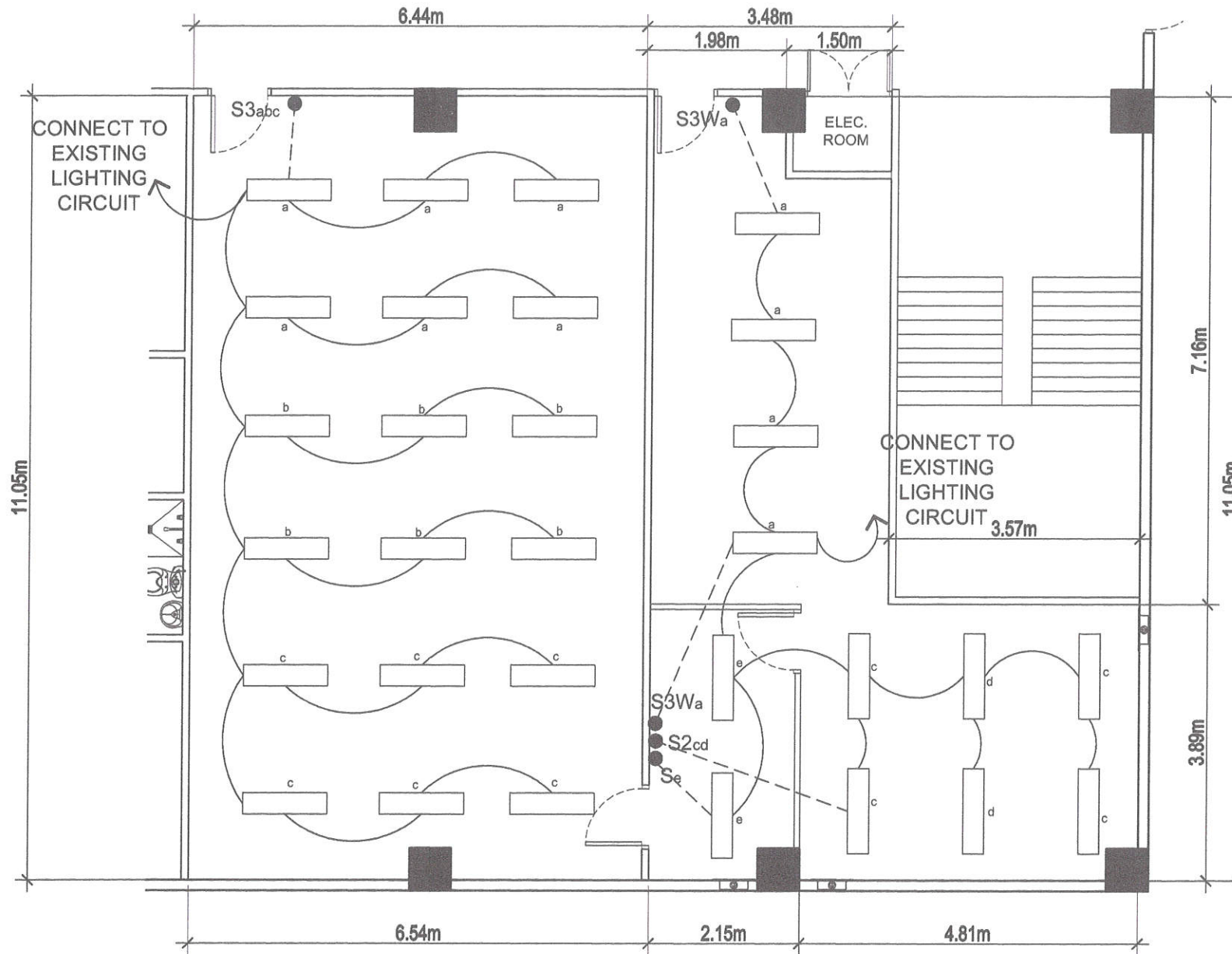
1 SECOND FLOOR - LIGHTING LAYOUT (PROPERTY & PROCUREMENT SECTION) SCALE NTS
