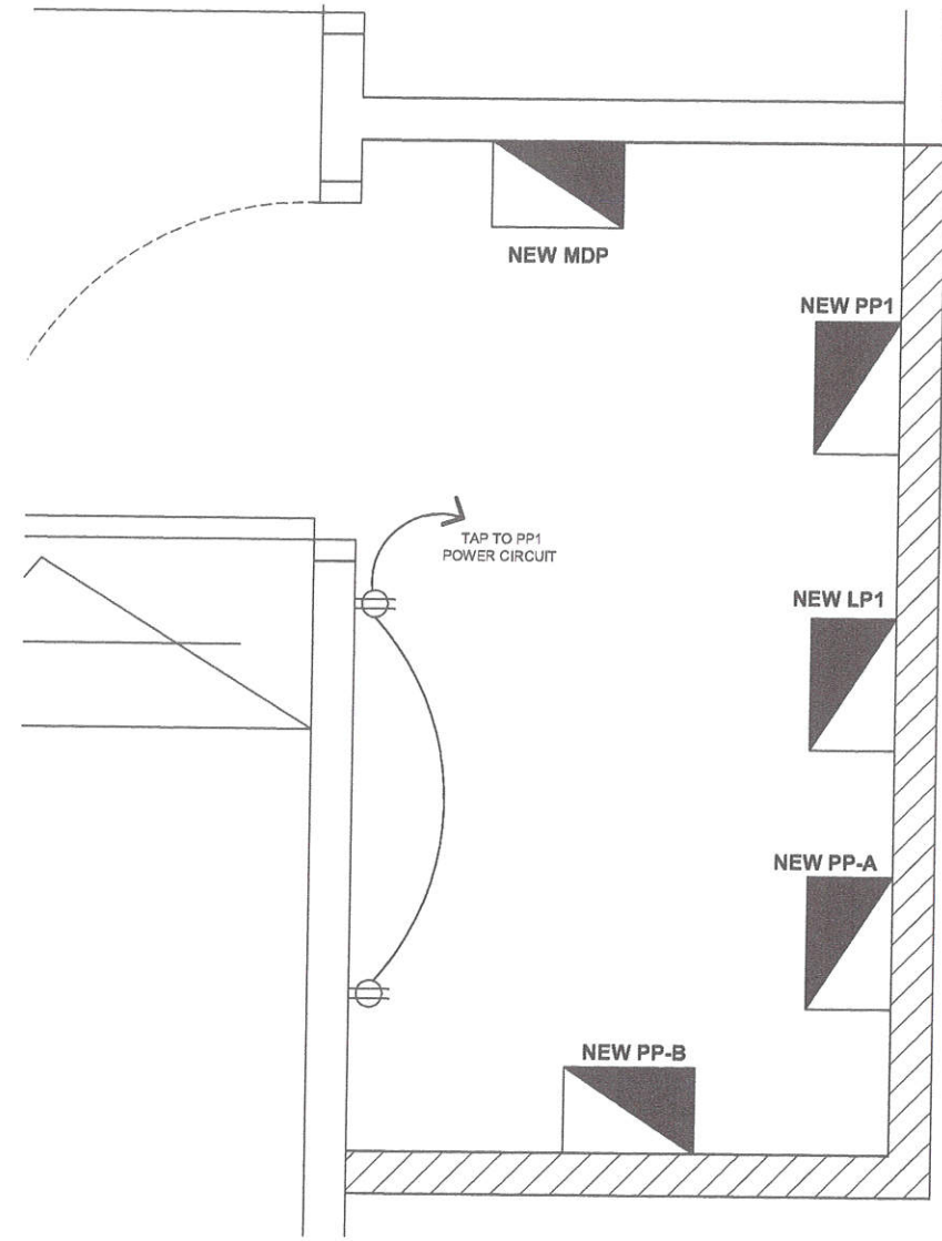
2 EXTENSION OF ELECTRICAL ROOM (POWER LAYOUT) SCALE NTS
