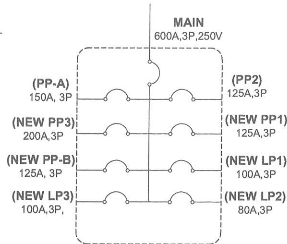
4 PANEL BOARD DIAGRAM SCALE NTS
