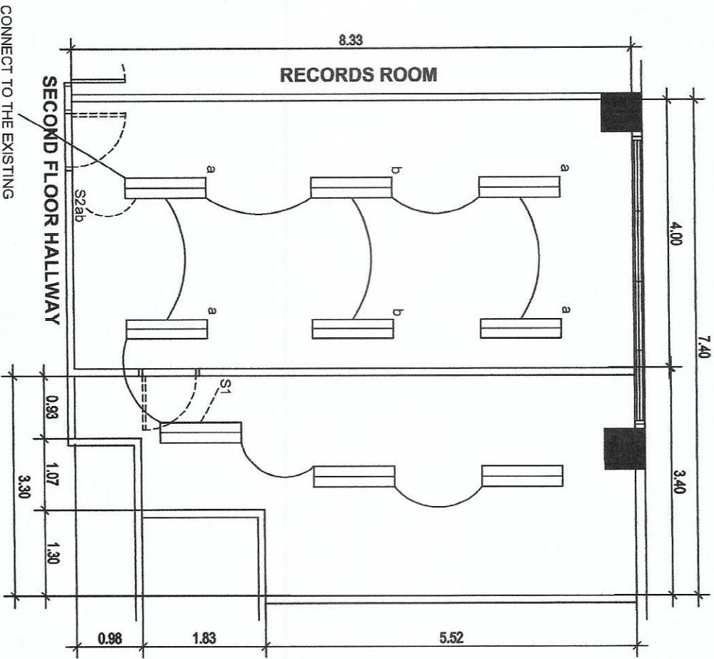
NART BLDG. - SECOND FLOOR PRINTING ROOM SCALE 1/100 NTS
