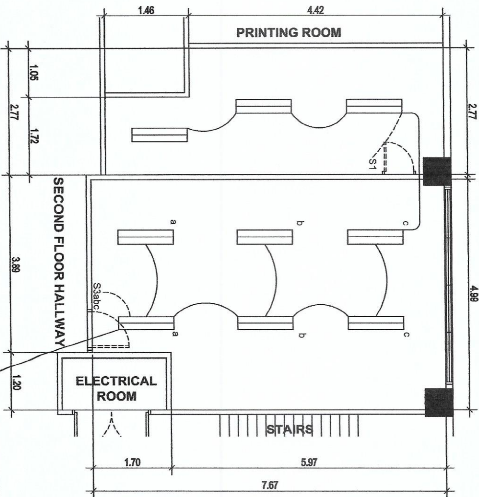
NART BLDG. - SECOND FLOOR CASHIER OFFICE SCALE 1/100 NTS
